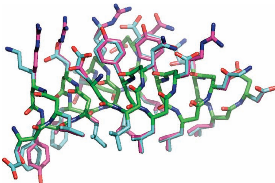
Figure 7. Comparison between experimental and computationally selected rotamers for the Zwit1f \beta -peptide scaffold using de novo \beta -peptide rotamer library. \beta_{314} backbone carbon atoms are shown in green, crystallographic side chain carbon atoms shown in blue and computationally selected rotamers shown in magenta. Oxygen and nitrogen atoms are shown in red and blue respectively. Note the good identity and rotameric agreement between 6 of the 8 core \beta -homoLeucines and 3 of 4 aromatic residues.
