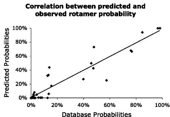
Figure 2. Comparison between predicted and observed rotamer probabilities of \alpha -helical rotamers (ILVFIYST), R = 0.946 . Optimized Boltzmann temperature of 450 K shown. Correlation of remaining \alpha -helical rotamers (CMWDENQHKR) which include extended side chains, R = 0.568 .
