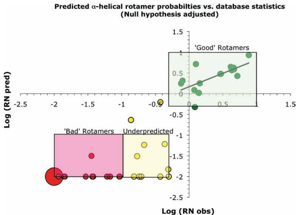
Figure 3. \log (predicted probabilities/null probability) vs \log (database probabilities/null probability) for the \alpha -helix ( \alpha AA residues VILSTFY, Boltzmann temperature 450^\circ for predicted probabilities). Green points are “good” predicted rotamers, RN_{\text{obs}} > 0.5 (the majority of which are over-represented when compared to the null hypothesis expectations); yellow points are “underpredicted” rotamers, RN_{\text{obs}} = 0.1\text{--}0.5 ; red points are rotamers that are ranked poorly, RN_{\text{obs}} < 0.1 (the point at -2, -2 represents 11 unique rotamer evaluations and is sized accordingly). Predicted probabilities with RN_{\text{obs}} < 0.01 are plotted at \log(RN_{\text{obs}}) = -2 .
