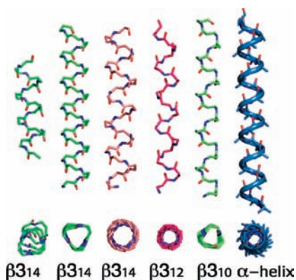
Figure 4. Various \beta -peptide helix motifs. From left to right: \beta_{314} helix from crystal structure, 22 energy minimized \beta_{314} 3.0 helix, \beta_{314} QM minimized \beta_{314} helix, 73 \beta_{312} helix, 77 and \beta_{310} helix. 76 Note the direction of the carbonyl groups in the \beta_{312} helix. Side-chain and hydrogen atoms omitted for clarity. \alpha -Helix shown for comparison at right.
