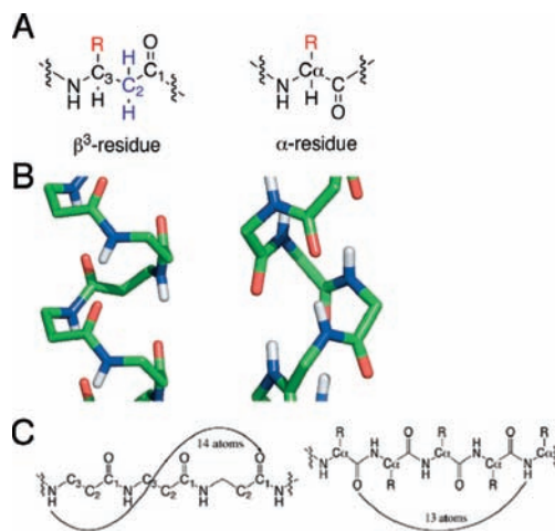
Figure 1. (A) backbone units for a \beta^3 AA (left) and \alpha AA (right) peptides. (B) Wireframe of \beta^3_{14} helix (left) and \alpha -helix (right, nonpolar hydrogens omitted for clarity, atoms colored by elemental type: carbon (green), oxygen (red), nitrogen (blue), and hydrogen (white)). (C) Hydrogen-bonding patterns for each structural motif. Note the direction of the carbonyl group in each subunit. The carbonyl points in the opposite direction in some \beta^3 AA peptide helices from that in the \alpha -helix.
