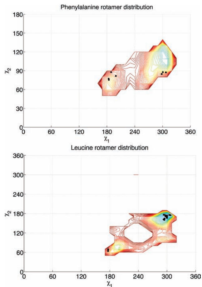
Figure 6. Contour plot of \chi_1/\chi_2 dependent rotamer probabilities for \beta^3 homoleucine and \beta^3 homophenylalanine in the \beta_{314} 3.0 rotamer library. The negative logs of rotamer probabilities are indicated via the contour map, in 10^5 \times 10^5 bins. Experimental rotamers from the crystal structure 22 are overlaid (black dots).
