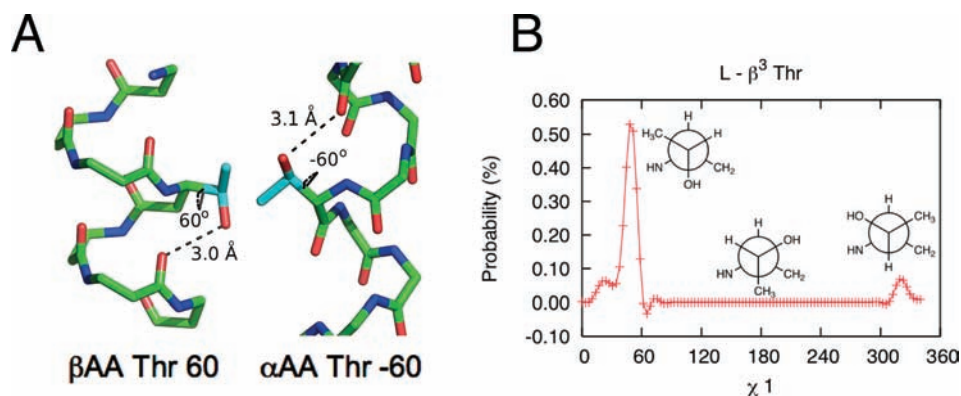
Figure 8. (A) \beta_{314} helix and \alpha -helix each with the threonine side chain. The preferred rotamer for each scaffold is shown, g^+ for \beta_{314} helix and g^- for the \alpha -helix. (B) Rotameric probabilities for \beta^3 substituted threonine. (Newman projections shown in inset.)
