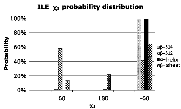
Figure 5. \chi_1 rotamer distributions for the isoleucine side chain in the context of the \alpha -helix, \beta -sheet, \beta_{314} helix, and the \beta_{312} helix. \alpha -Helix and \beta -sheet rotameric preference derived from a binned backbone dependent rotamer library for each secondary structure.
